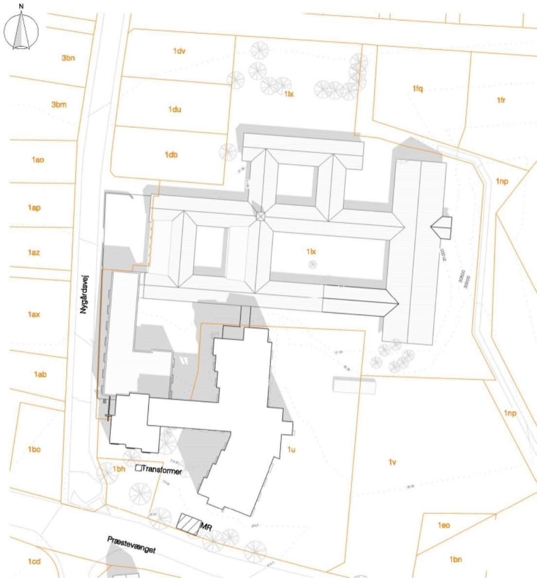
Situationsplan
